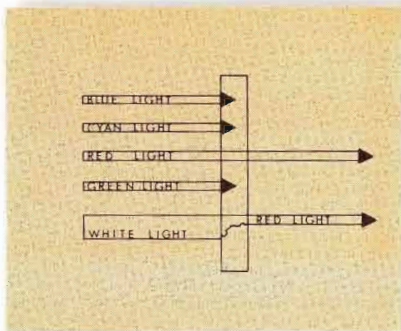
Fig. 4 A dense color filter will only allow its color to pass.
