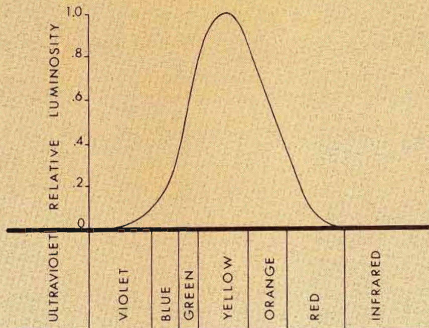
Fig. 5 Colors as they would look if they were laid out in a straight line.
