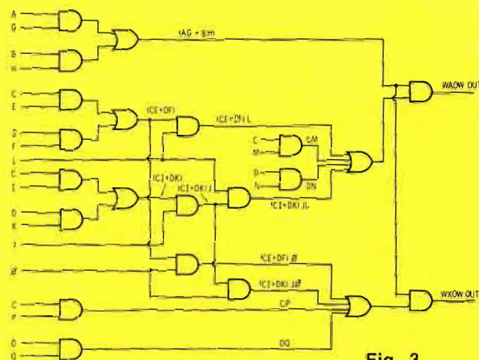
Fig. 3 ID logic arrangement.
